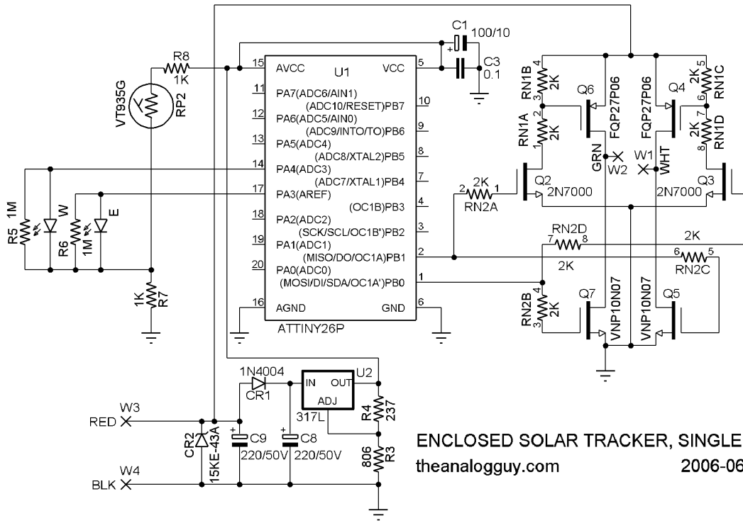
SCHEMATIC DIAGRAM OF THE INSIDES OF THE EST1
